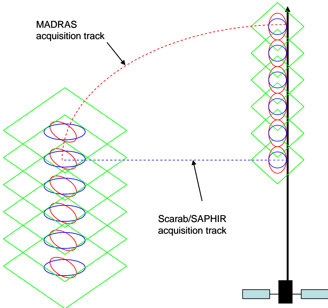
Figure 6.2-6: Pixel representation on ground of the 3 instruments
